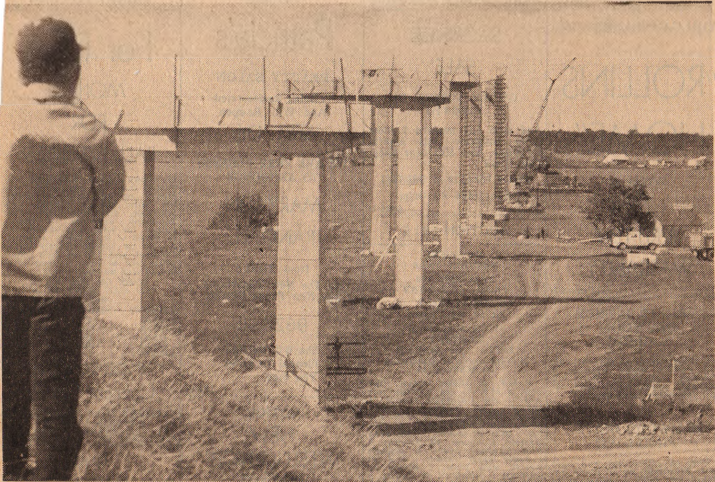
Young visitors as well as old are viewing the new Green Point bridge "The Quinte Skyway" these days. Nearly every Sunday sees a crowd of interested persons inspecting progress of construction. Approaches are nearly finished on the Green Point (Prince Edward side) and sodding has been done.
